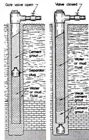
Figure 2. Cementing by casing method using single plug between grout column and drilling fluid. Plug and grout are forced out of bottom of pipe; grout then moves upward in annular space.
