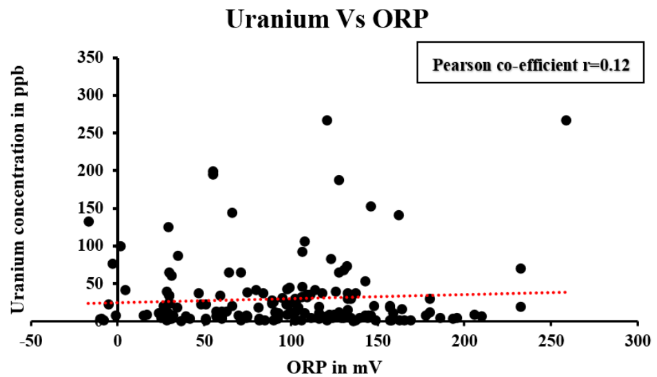
Figure 6. Pearson correlation between uranium concentration and ORP.
