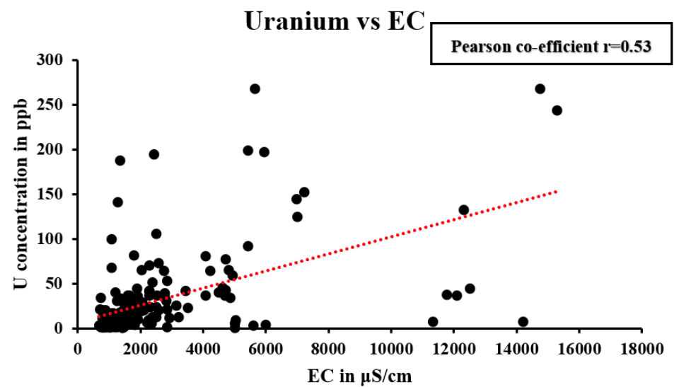
Figure 7. Pearson correlation between uranium concentration and EC.
