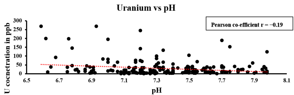
Figure 8. Pearson correlation between uranium concentration and pH.
