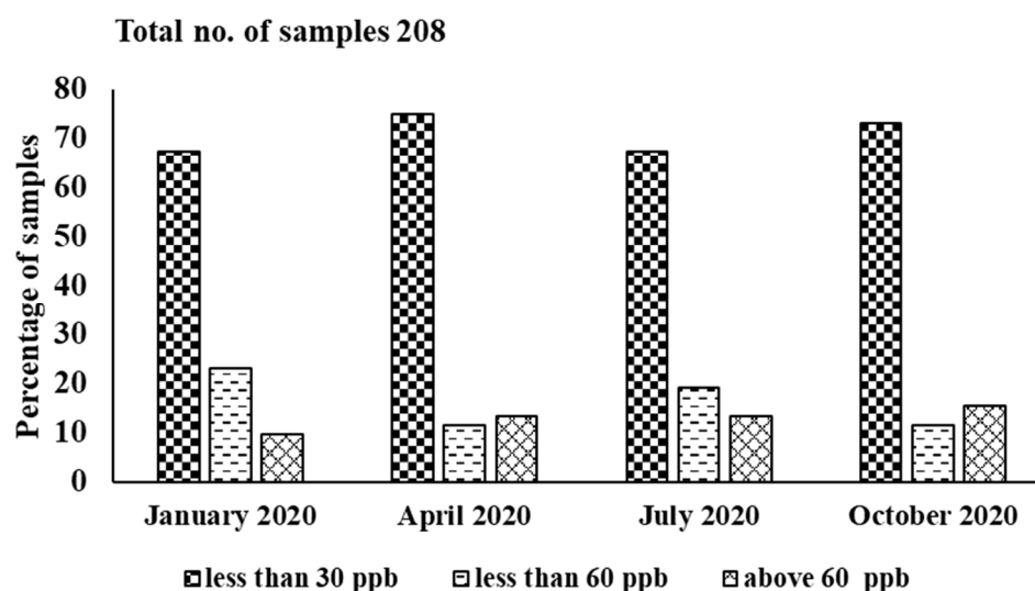
Figure 5. Range of uranium concentration in groundwater.
