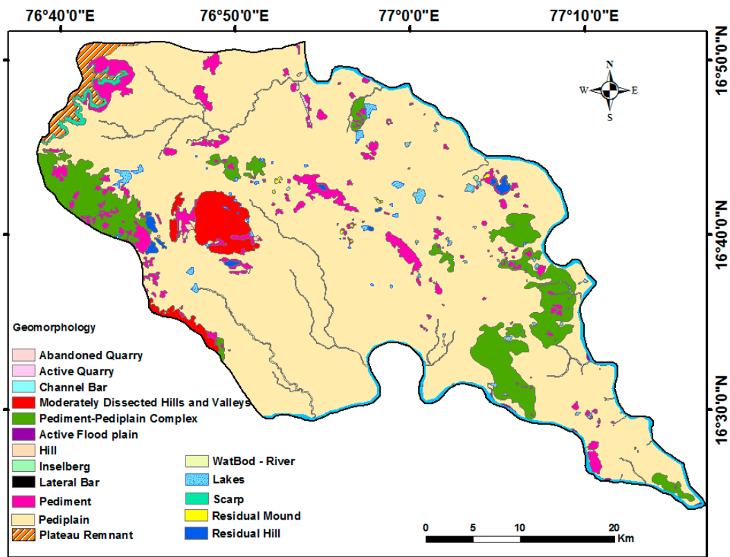
Figure 4. Geomorphology of the study area.
