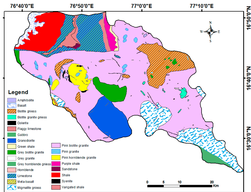
Figure 2. Lithology of the study area.
