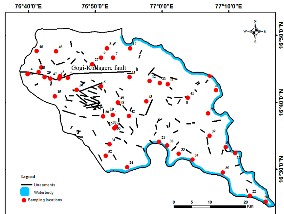
Figure 3. Lineaments and sampling well locations in the study area.
