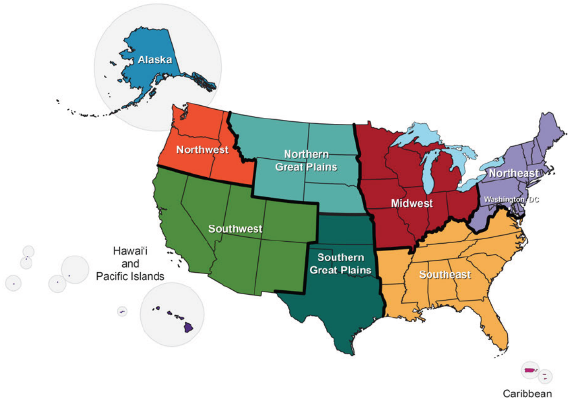
2 Figure 1. Map of the ten regions of the United States used throughout the Climate Science 3 Special Report. Regions are similar to that used in the Third National Climate Assessment except 4 that 1) the Great Plains are split into the Northern Great Plains and Southern Great Plains, and 2) 5 the Caribbean islands have been split from the Southeast region. (Figure source: adapted from 6 Melillo et al. 2014).
