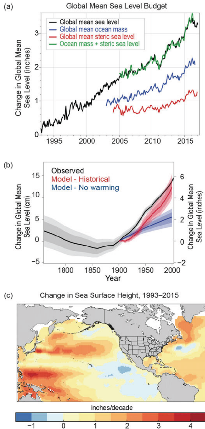
1 2 Figure 12.3: (a) Contributions of ocean mass changes from land ice and land water storage 3 (measured by satellite gravimetry) and ocean volume changes (or steric, primarily from thermal 4 expansion measured by in situ ocean profilers) and their comparison to global mean sea level 5 (GMSL) change (measured by satellite altimetry) since 1993. (b) An estimate of modeled GMSL 6 rise in the absence of 20th century warming (blue) and from the same model with observed 7 warming (red), compared to observed GMSL change (black). Heavy/light shading indicates the
